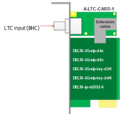
A-LTC-CARD-1 mounted on DELTA-3G-elp-d 4c, DELTA-3G-elp-d 8c, DELTA-3G-elp-key-d 2K or DELTA-3G-elp-key-d 4K DELTA-ip-st2022-6
