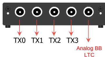
FLEX-hmi 10 / 01 Front View
